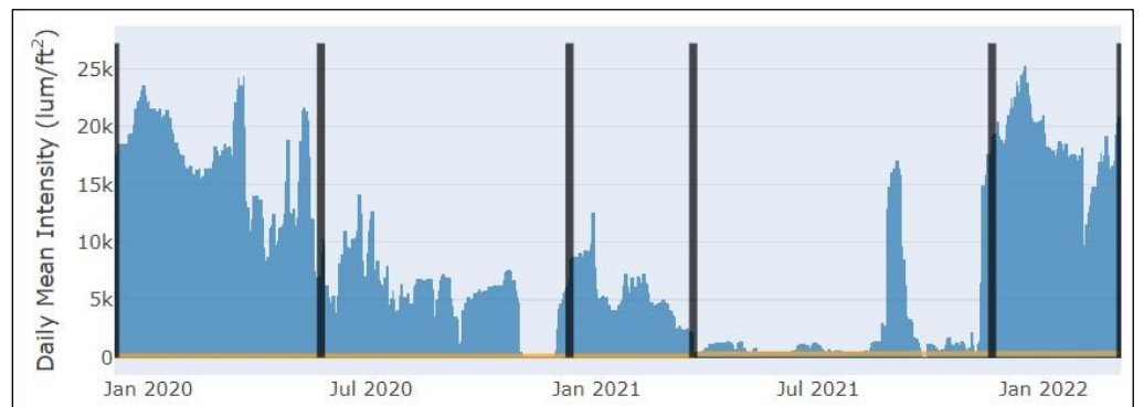
Intermittent stream reach Dry Comal Creek, New Braunfels, TX
