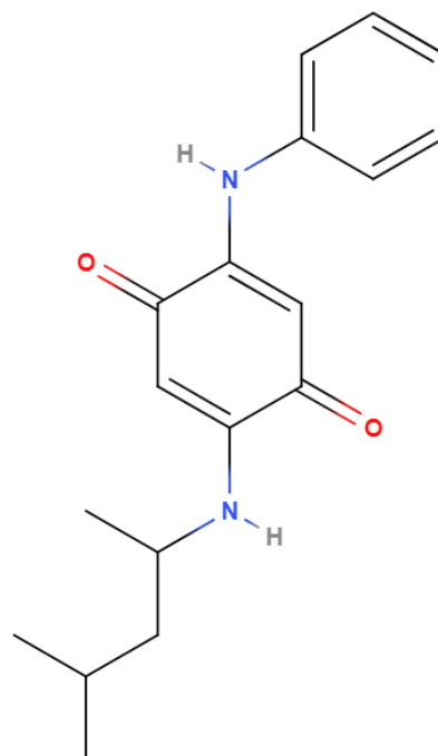
6PPD-quinone
