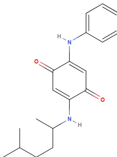
7PPD-quinone
