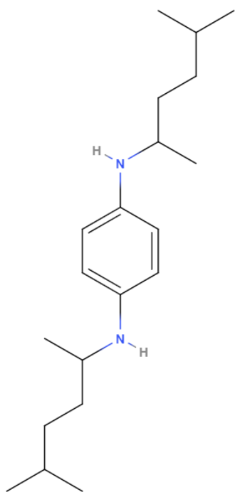
77PD
