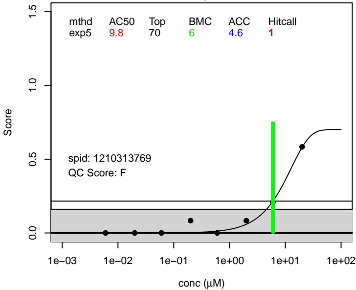
1-(Perfluorooctyl)propane-2,3-diol score.any ; 94159-84-9
