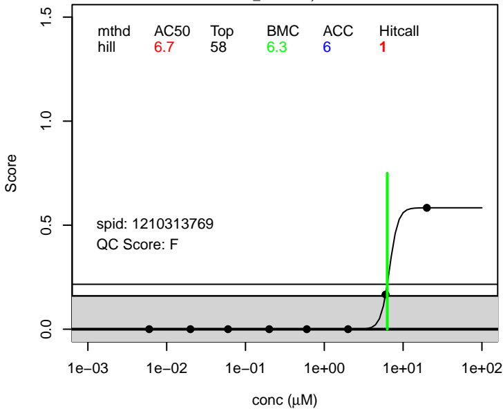
1-(Perfluorooctyl)propane-2,3-diol score.edema ; 94159-84-9
