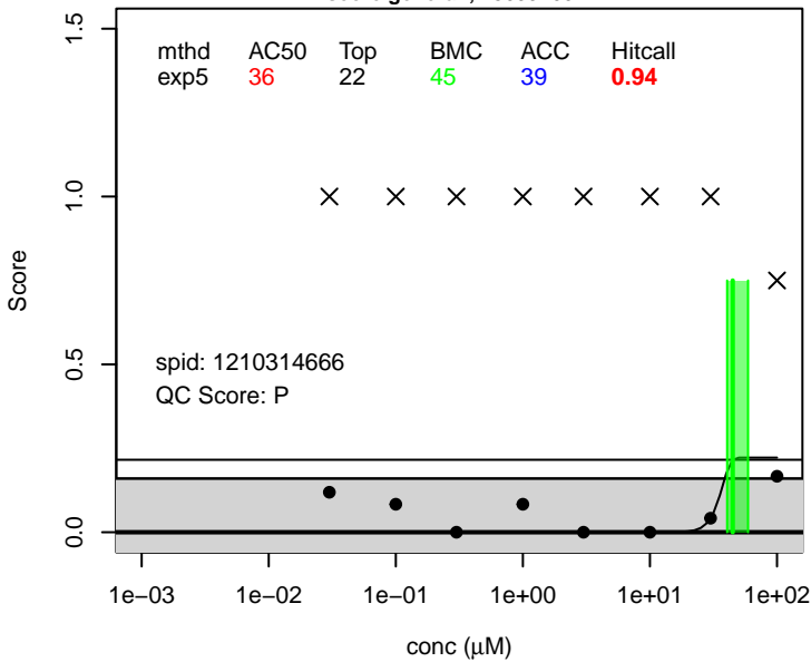
7:3 FTOH score.general ; 25600-66-2
