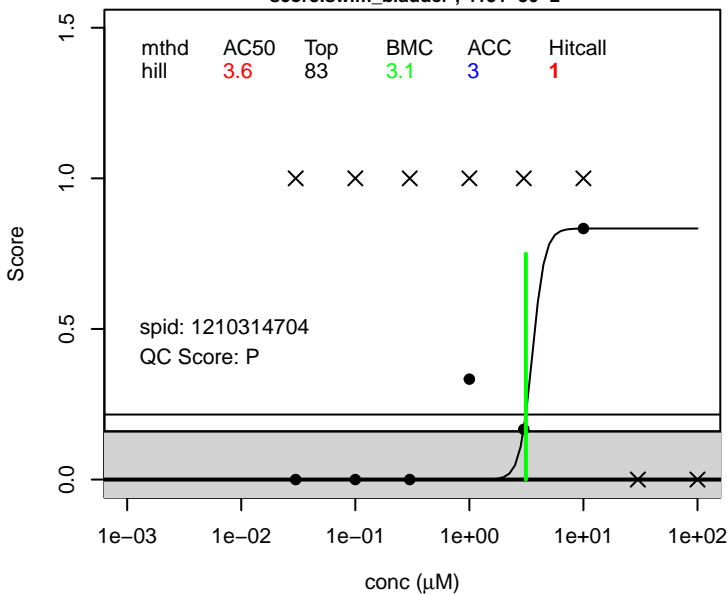
NEtFOSA score.swim_bladder ; 4151-50-2
