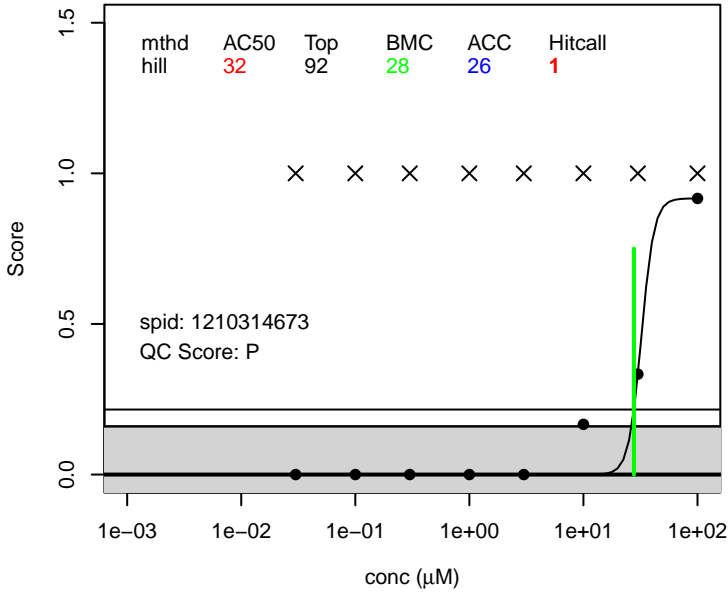
((2,2,3,3-Tetrafluoropropoxy)methyl)oxirane score.any ; 19932-26-4
