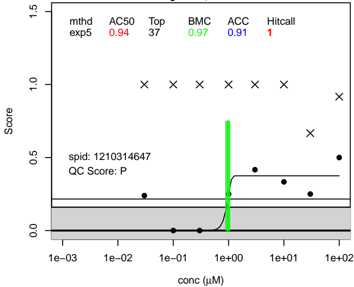
N-MeFOSA score.general ; 31506-32-8
