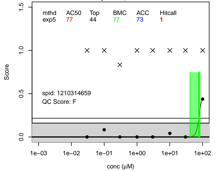
3H-Perfluoro-2,2,4,4-tetrahydroxypentane score.any ; 77953-71-0
