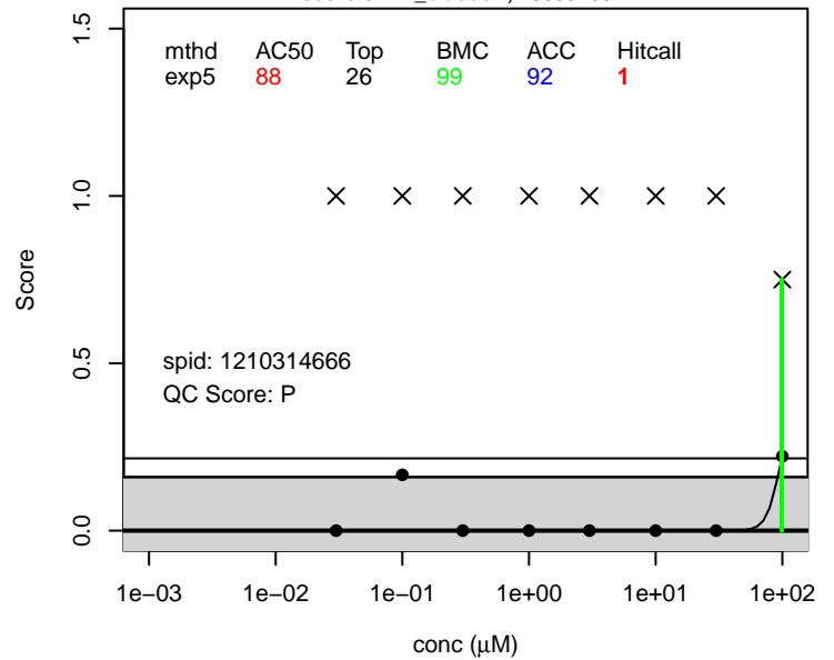
7:3 FTOH score.swim_bladder ; 25600-66-2
