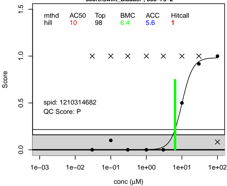
CI-PFNA score.swim_bladder ; 865-79-2
