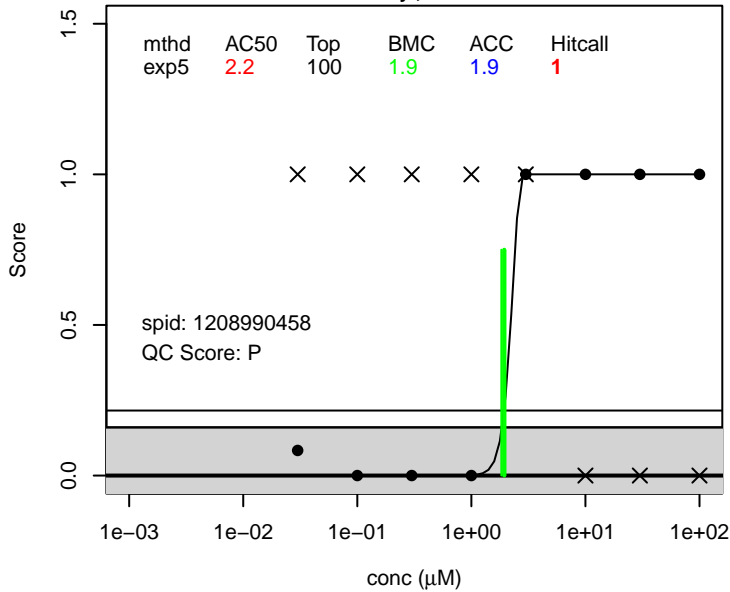
Perfluoropinacol score.any ; 918-21-8
