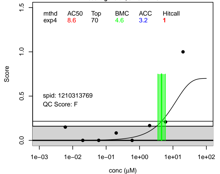
1-(Perfluorooctyl)propane-2,3-diol score.general ; 94159-84-9
