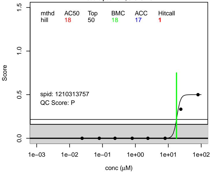
PFHpS score.position ; 375-92-8
