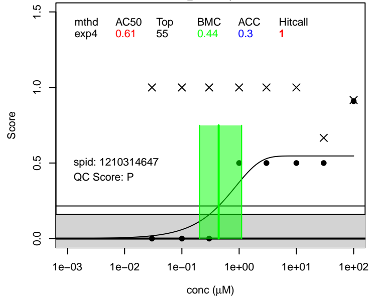
N-MeFOSA score.swim_bladder ; 31506-32-8
