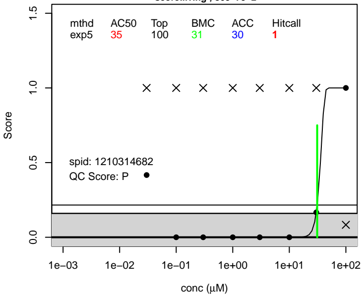
CI-PFNA score.swim_bladder ; 865-79-2
