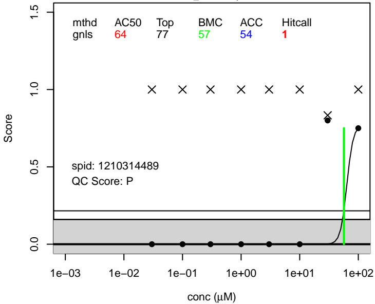
6:1 FTOH score.living ; 375-82-6
