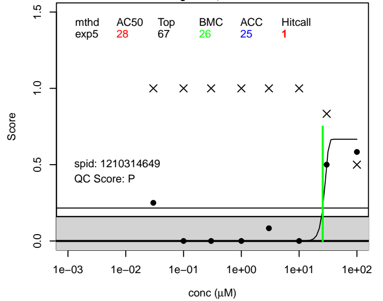
(Heptafluorobutanoyl)pivaloylmethane score.craniofacial ; 17587-22-3
