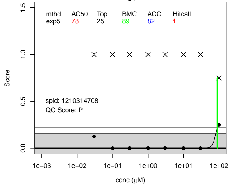
1H,1H-Perfluoro-3,6,9-trioxadecan-1-ol score.general ; 147492-57-7
