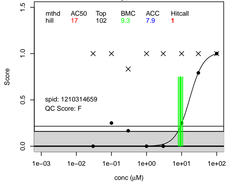
7:3 FTOH score.swim_bladder ; 25600-66-2
