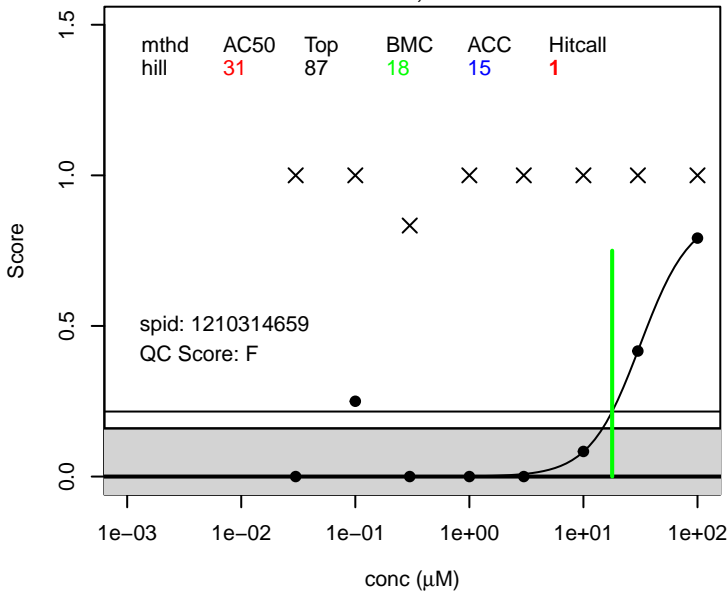
3H-Perfluoro-2,2,4,4-tetrahydroxypentane score.blood_pooling ; 77953-71-0
