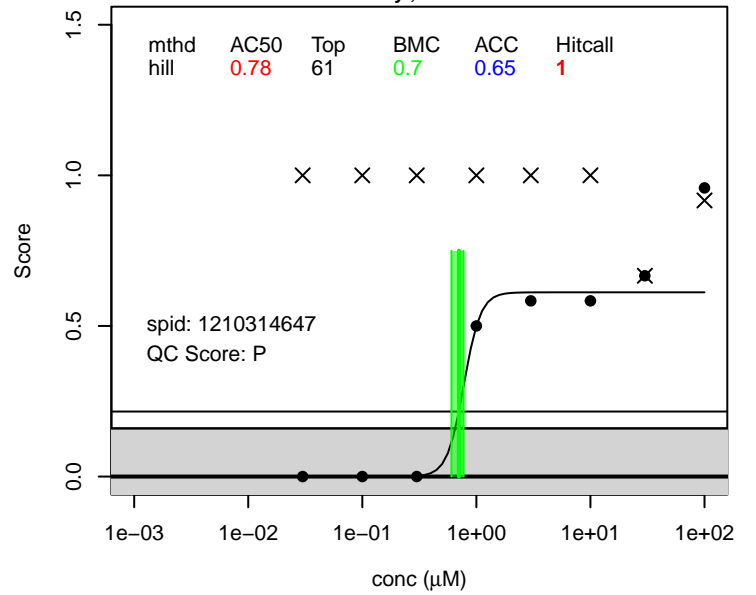
(Heptafluorobutanoyl)pivaloylmethane score.general ; 17587-22-3
