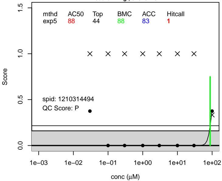
6:1 FTOH score.living ; 375-82-6
