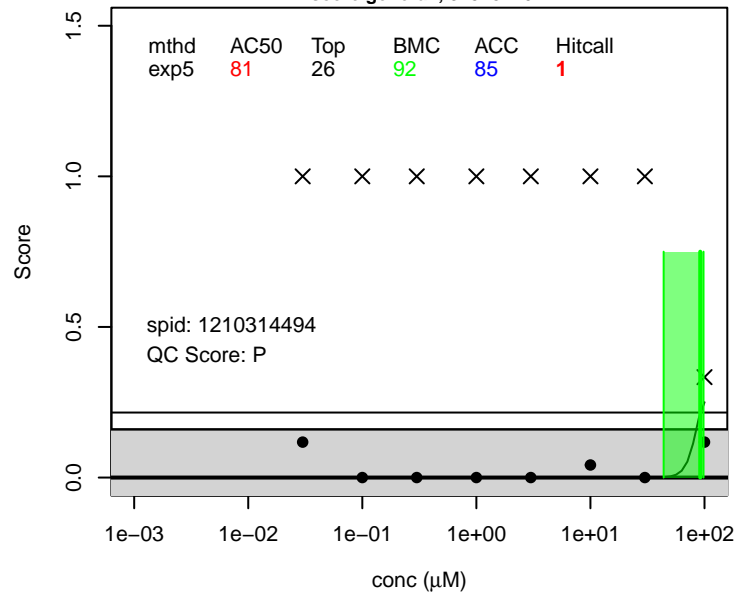
6:1 FTOH score.general ; 375-82-6
