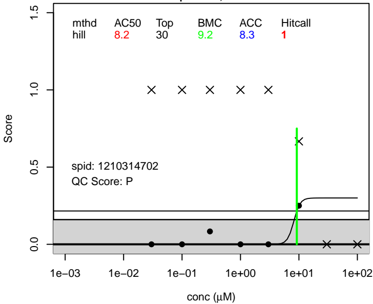
NEtFOSA score.living ; 4151-50-2
