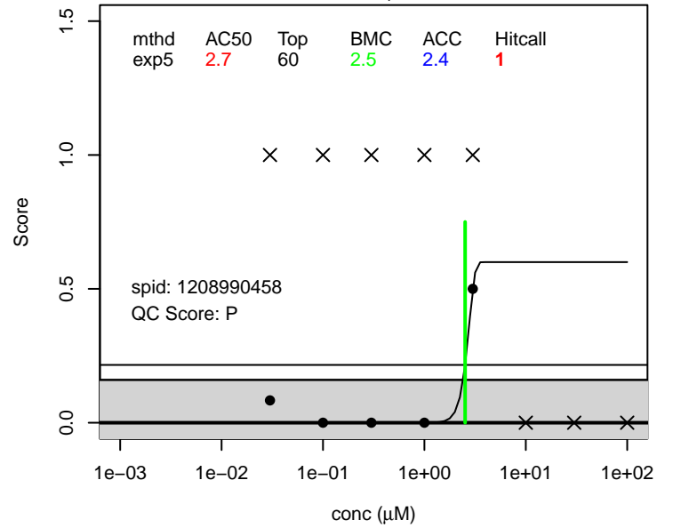
Perfluoro-1,4-diiodobutane score.general ; 375-50-8
