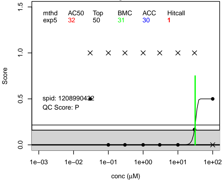
H-PFUnA score.general ; 1765-48-6
