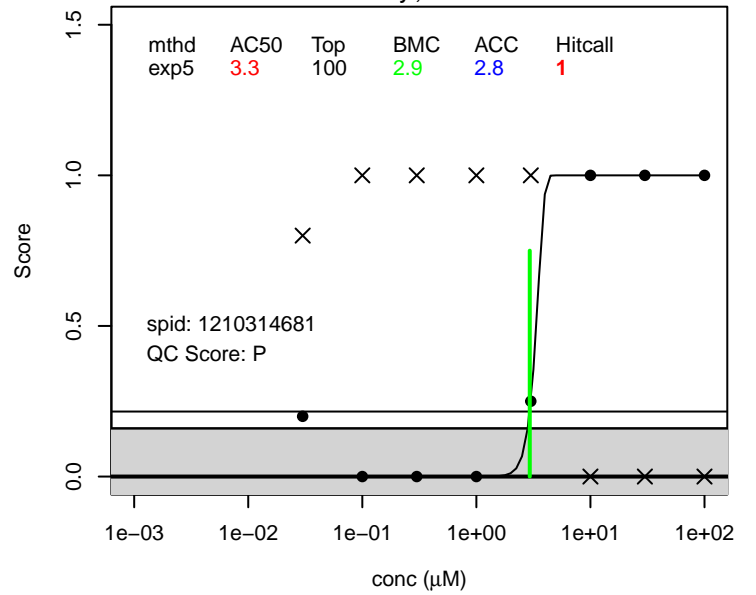
PFUnDA score.any ; 2058-94-8
