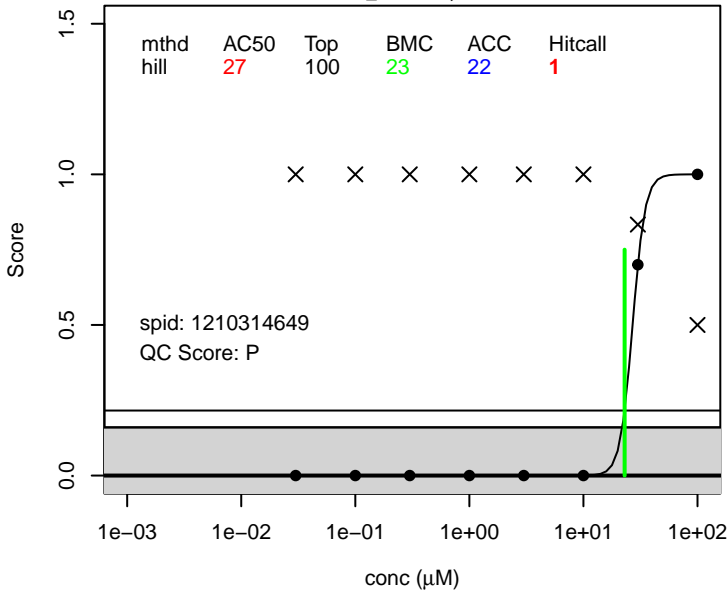
(Heptafluorobutanoyl)pivaloylmethane score.swim_bladder ; 17587-22-3
