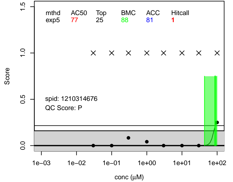
5:3 PFOA score.general ; 914637-49-3
