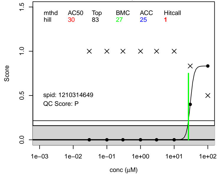
(Heptafluorobutanoyl)pivaloylmethane score.craniofacial ; 17587-22-3
