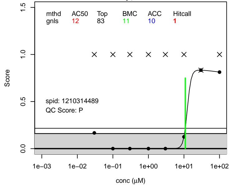
6:1 FTOH score.general ; 375-82-6
