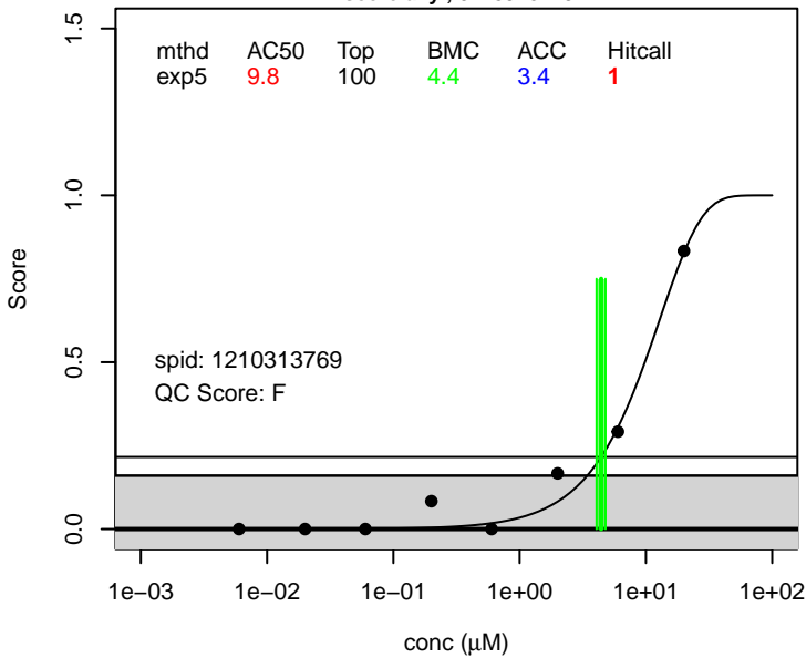
1-(Perfluorooctyl)propane-2,3-diol score.any ; 94159-84-9
