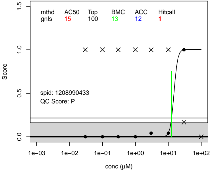
H-PFUnA score.any ; 1765-48-6
