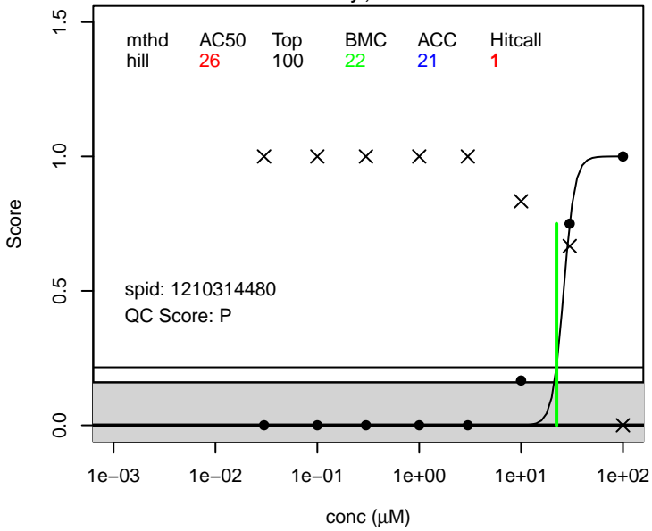
1-Iodopentadecafluoroheptane score.swim_bladder ; 335-58-0
