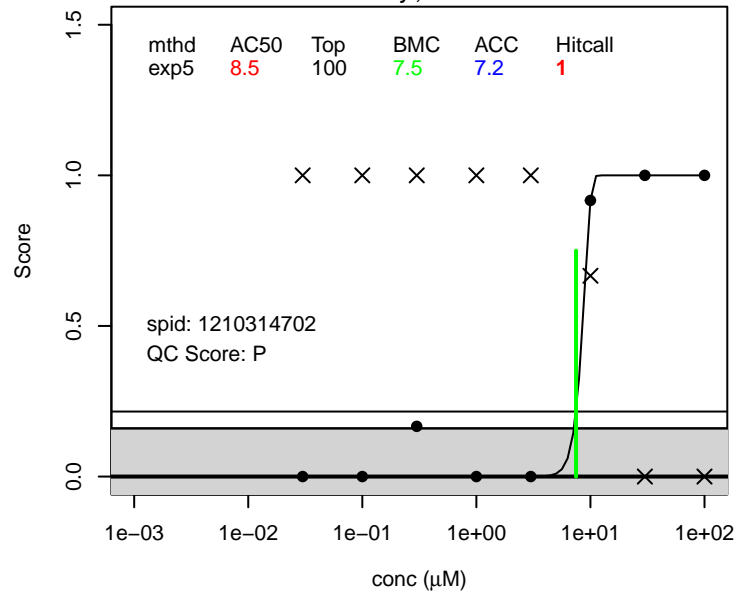
NEtFOSA score.general ; 4151-50-2
