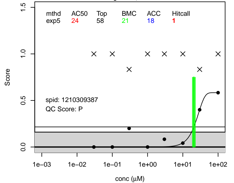
Perfluoro-1,4-diiodobutane score.general ; 375-50-8
