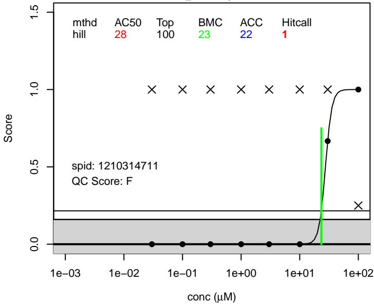
1H,1H-Perfluoro-3,6,9-trioxadecan-1-ol score.swim_bladder ; 147492-57-7
