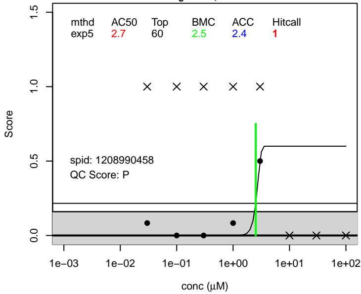
Perfluoropinacol score.craniofacial ; 918-21-8
