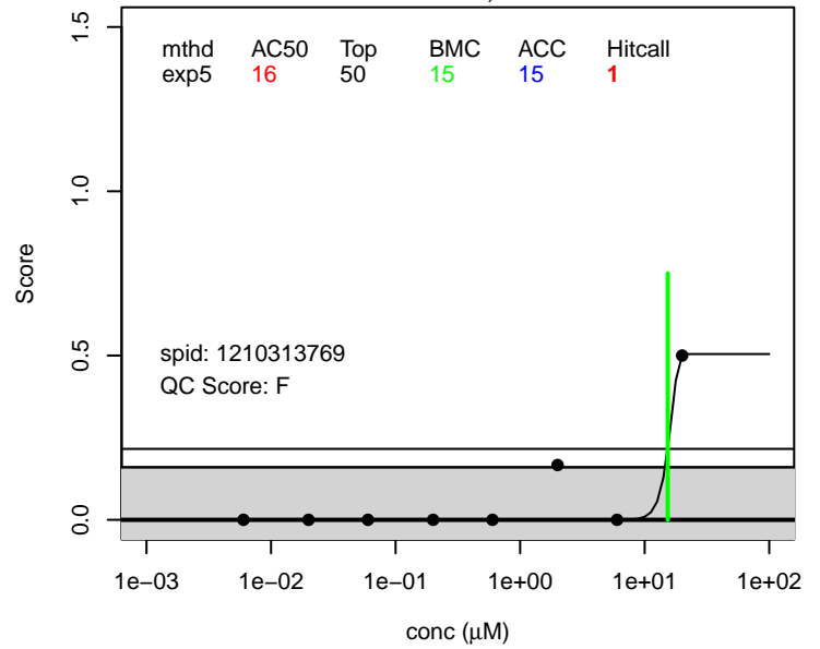
1-(Perfluorooctyl)propane-2,3-diol score.position ; 94159-84-9
