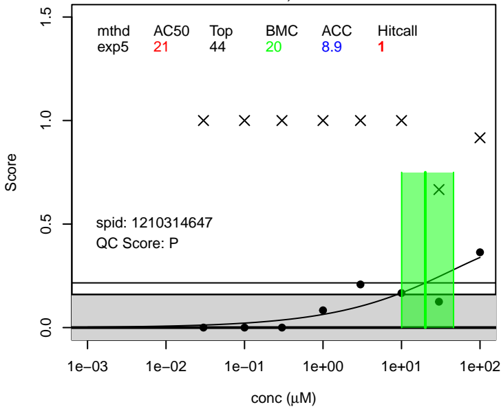
(Heptafluorobutanoyl)pivaloylmethane score.living ; 17587-22-3
