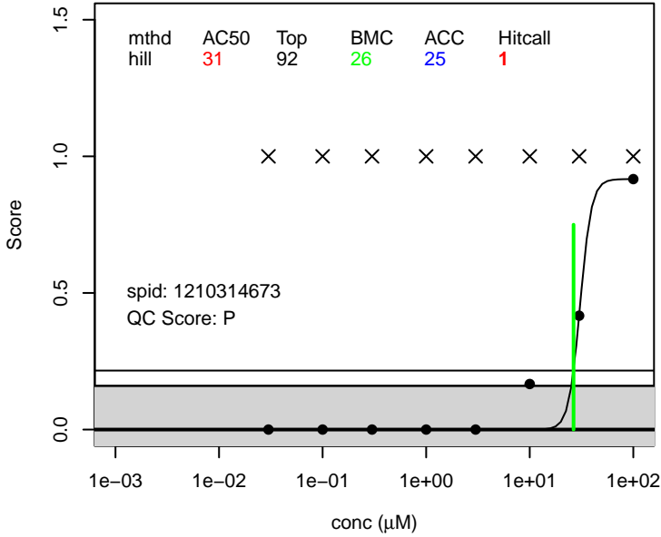
5:3 PFOA score.living ; 914637-49-3
