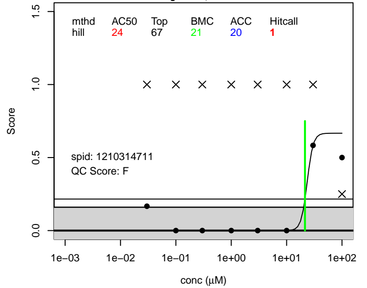
1H,1H-Perfluoro-3,6,9-trioxadecan-1-ol score.craniofacial ; 147492-57-7
