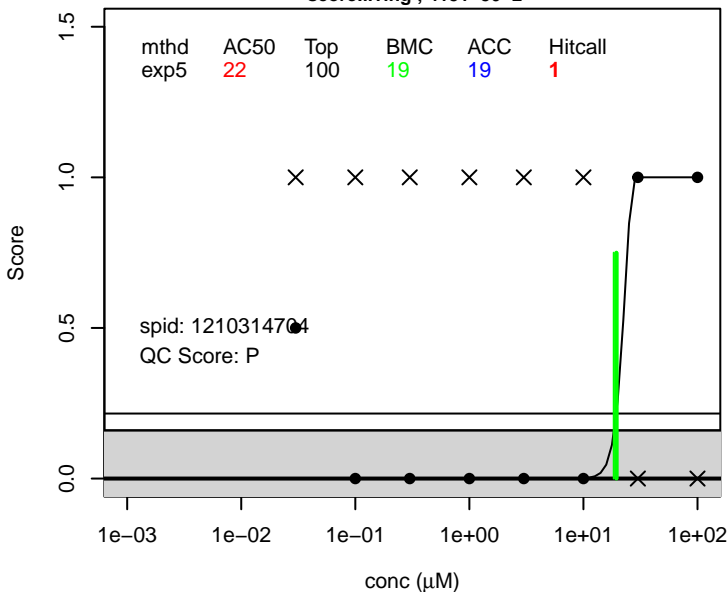
NEtFOSA score.swim_bladder ; 4151-50-2
