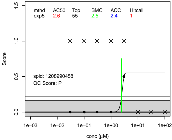
Perfluoropinacol score.any ; 918-21-8
