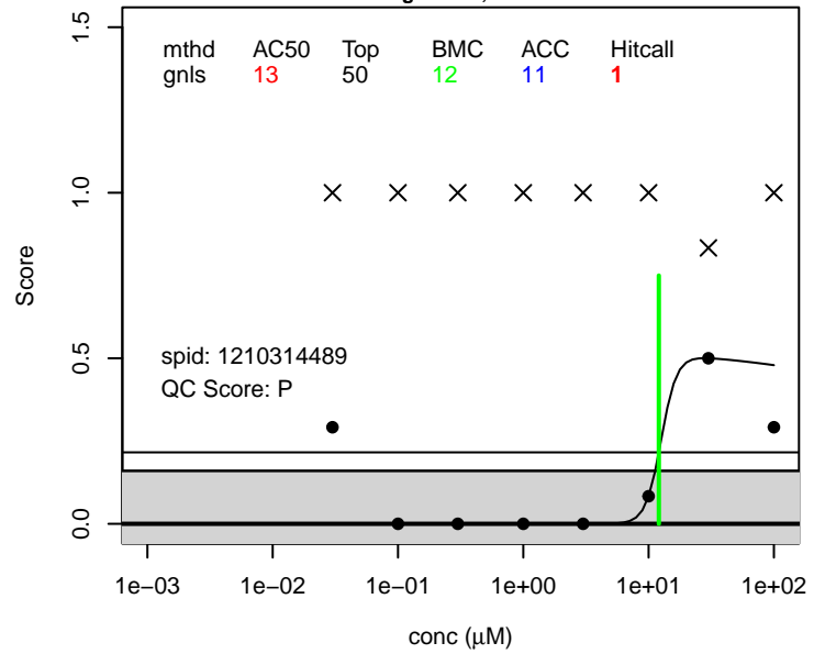
1-Iodopentadecafluoroheptane score.any ; 335-58-0
