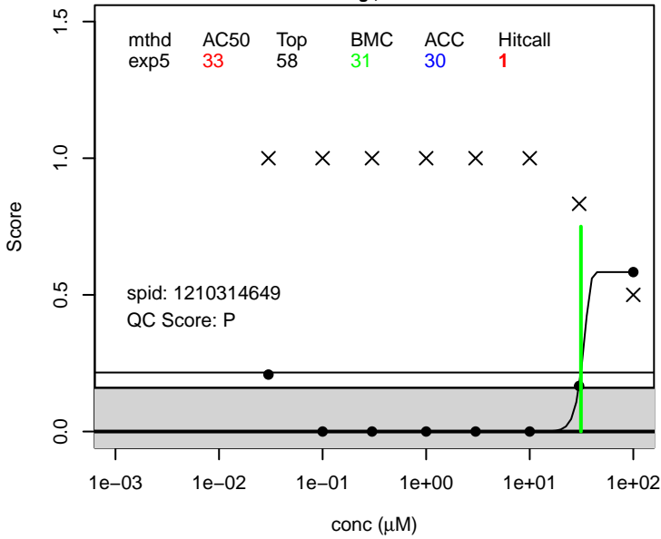
(Heptafluorobutanoyl)pivaloylmethane score.swim_bladder ; 17587-22-3
