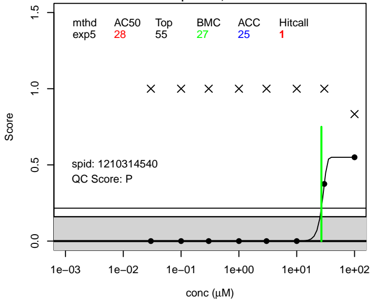
1,6-Diiodoperfluorohexane score.any ; 375-80-4
