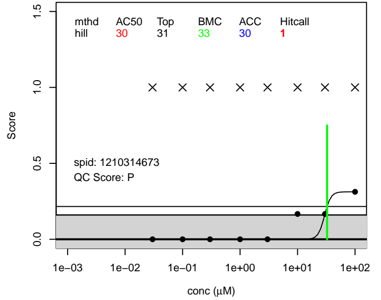
3:3 FTCA score.any ; 356-02-5
