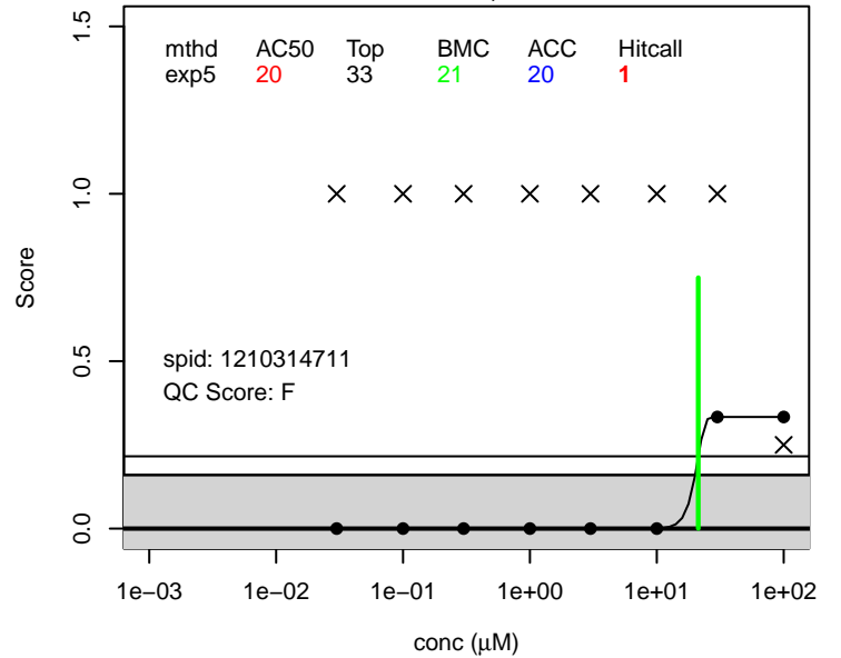
1H,1H-Perfluoro-3,6,9-trioxadecan-1-ol score.craniofacial ; 147492-57-7
