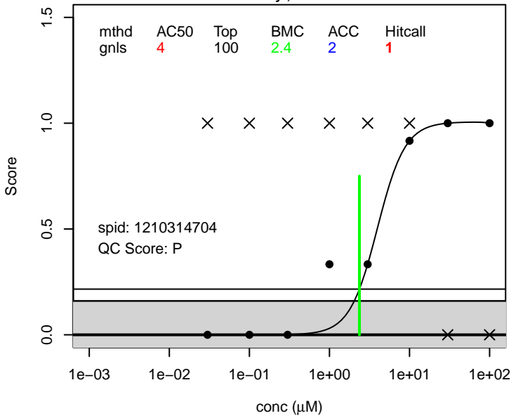
1H,1H-Perfluoro-3,6,9-trioxadecan-1-ol score.living ; 147492-57-7
