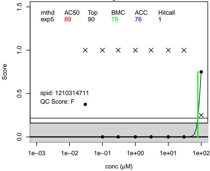
1H,1H-Perfluoro-3,6,9-trioxadecan-1-ol score.swim_bladder ; 147492-57-7
