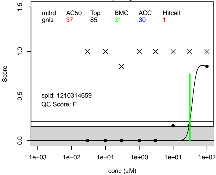
7:3 FTOH score.general ; 25600-66-2
