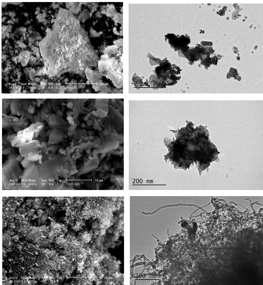
Figure 1. Physicochemical properties of nanohybrids. (A) SEM and TEM images, (B) Raman analysis of four types of nanohybrids, and (C) FT-IR analysis of four different types of NHs [Baek et al., 2018].
