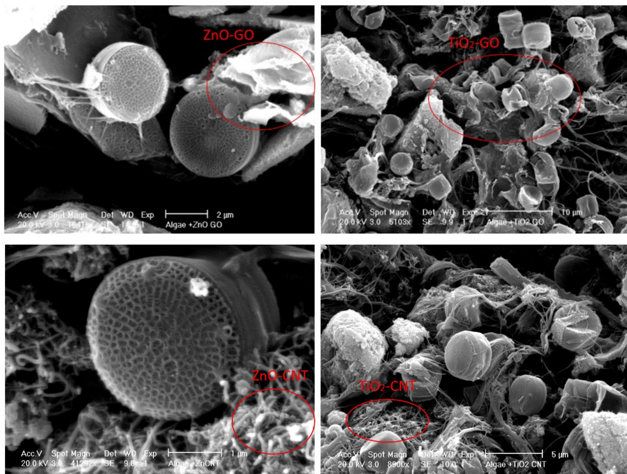
Figure 4. SEM images of four different types of NHs after exposure to T. pseudonana for 72 h.
