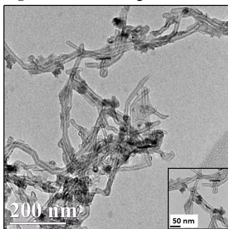
Figure 1b. TEM images of the CNT-Fe 3 O 4 NHs
